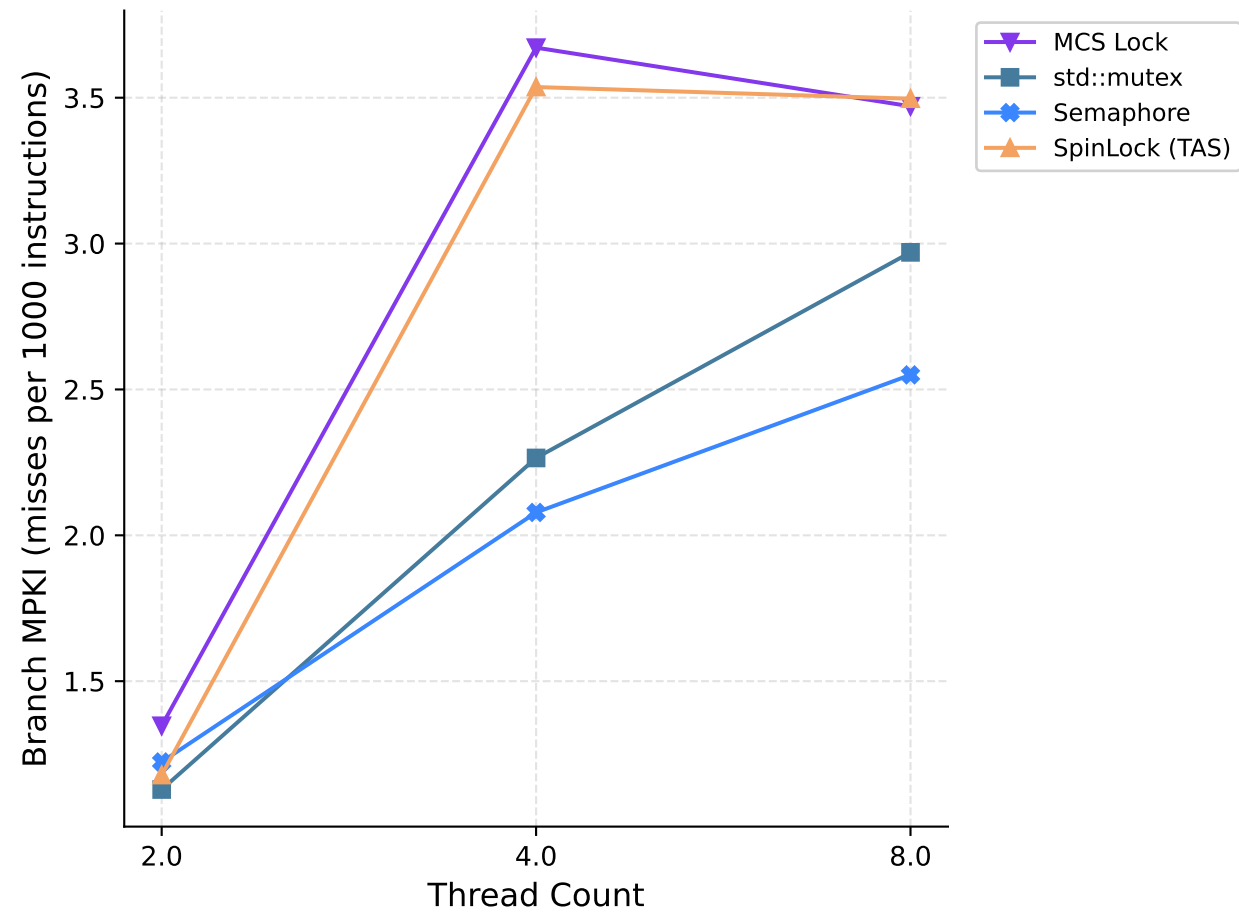
Branch MPKI vs Threads
