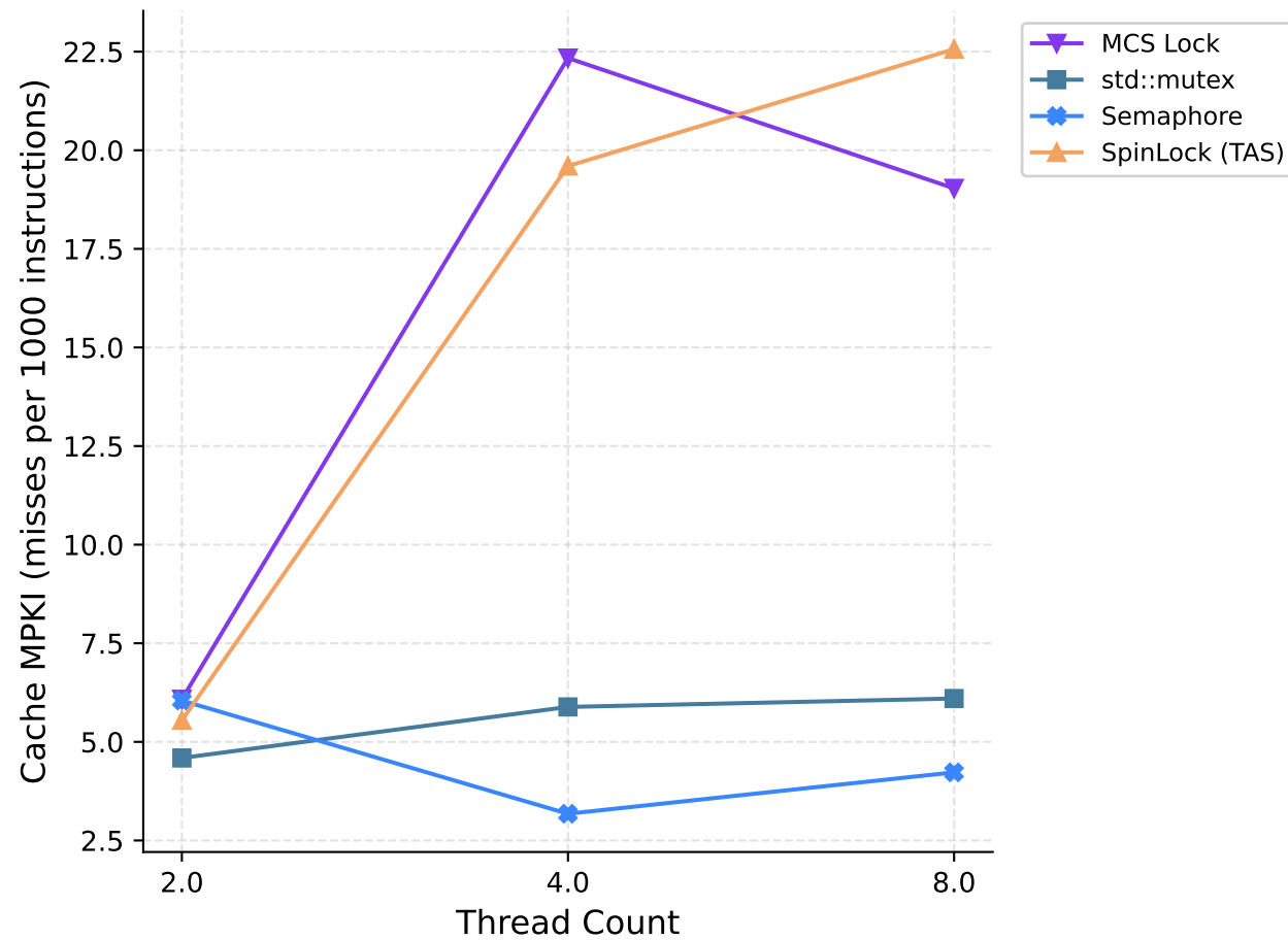
Cache MPKI vs Threads
